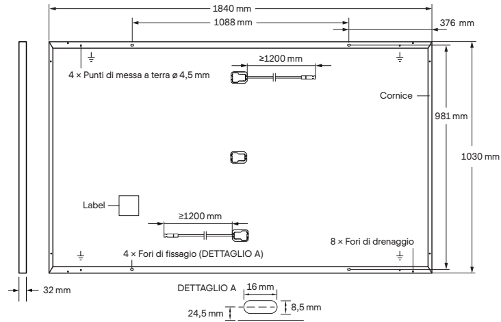
Fig. 1: Dimensioni d'ingombro (in mm) e componenti per Q.PEAK DUO ML-G9, Q.PEAK DUO BLK ML-G9, Q.PEAK DUO ML-G9+ e Q.PEAK DUO BLK ML-G9+
